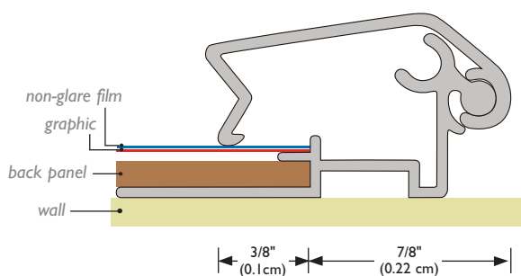
Standard frame with back panel:
