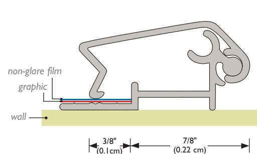
Optional bottom flat wall extrusion w/o back panel (only for mitered corners):
